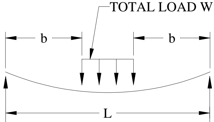
Figure 9 Beam Loading Conditions for Deflection Analysis
