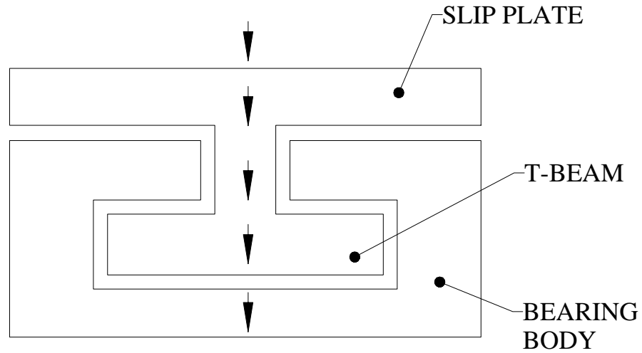
Figure 5 Load Path through a T-Film Bearing
