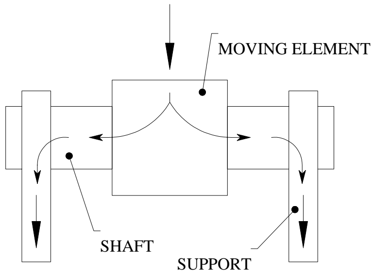
Figure 6 Load Path through a Journal Bearing
