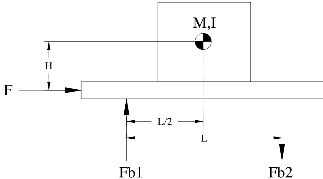
Figure 3b Free Body Diagram of Forces Acting on Slip Plate
