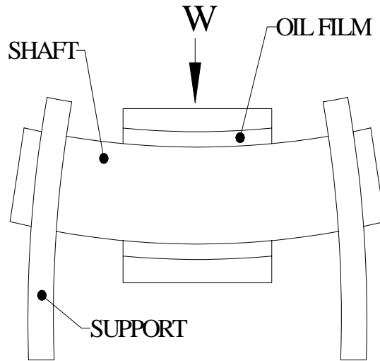
Figure 8a Journal Bearing Stiffness Model
