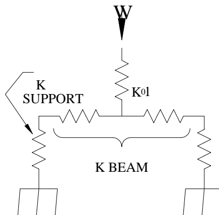
Figure 8b Spring Model of Journal Bearing
