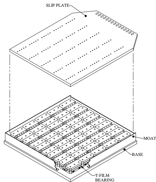
Figure 4 T-Film Table Assembly
