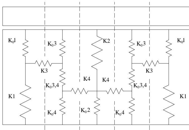
Figure 7b Spring Model of T-Film Bearing
